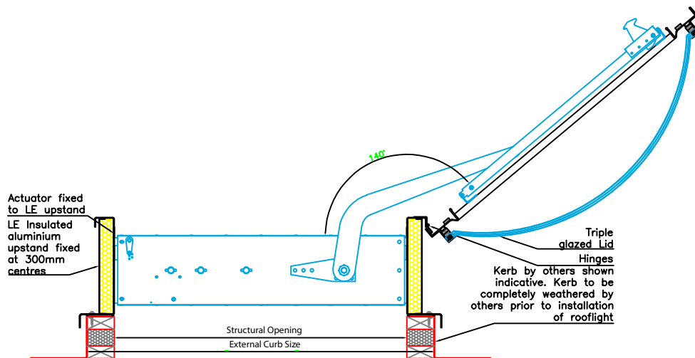
Section B-B Open Scale 1:10
