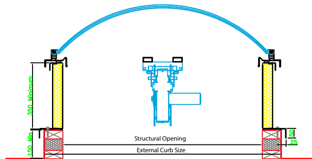
Section A-A Scale 1:10
